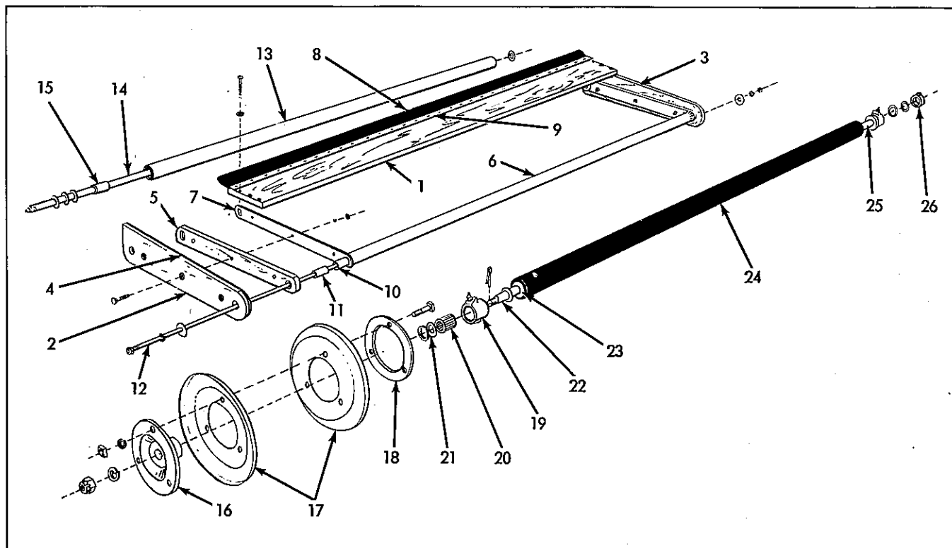
FLOATING FRAME & DRIVE ROLLER
