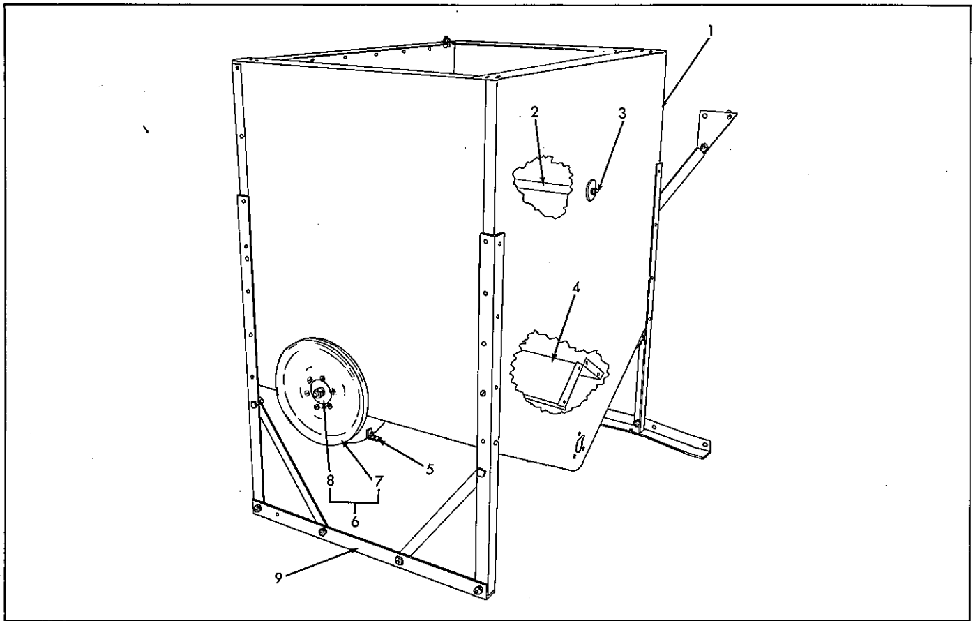
GRAIN BIN R.H. Rear View
