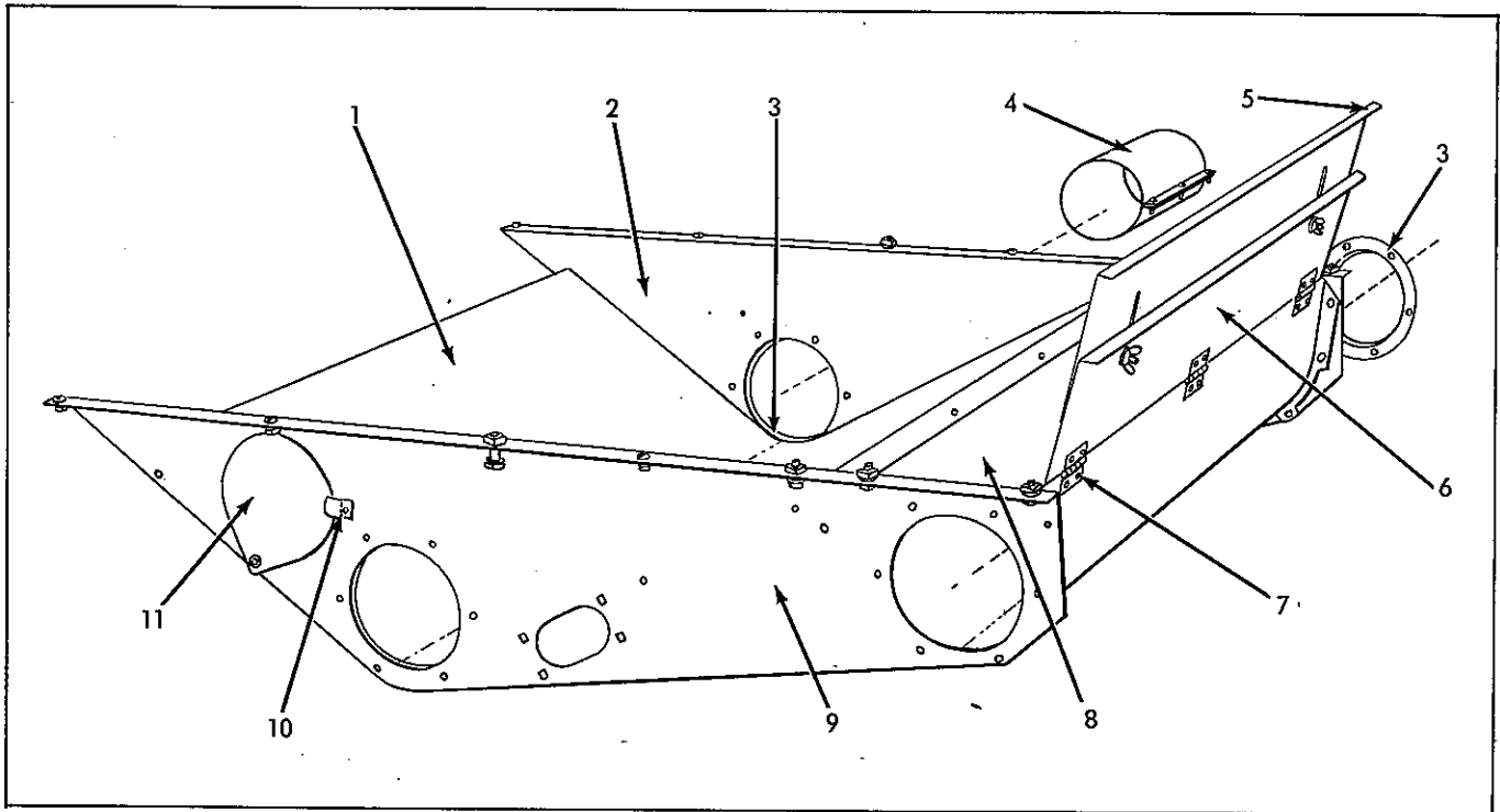
GRAIN & TAILINGS CONVEYOR HOUSING
