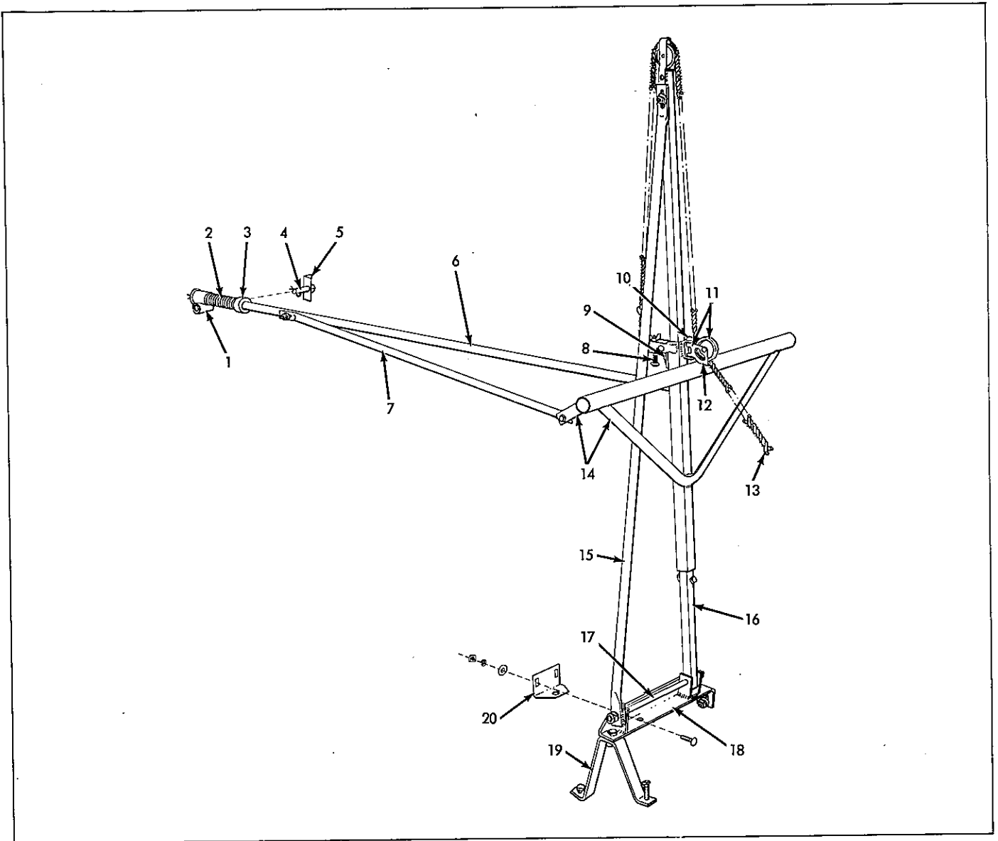
REEL SUPPORT POST
