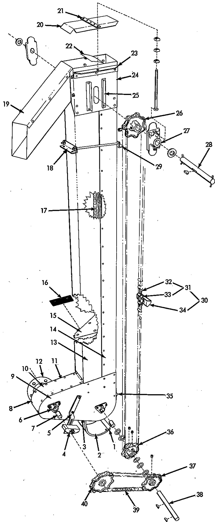
GRAIN ELEVATOR
