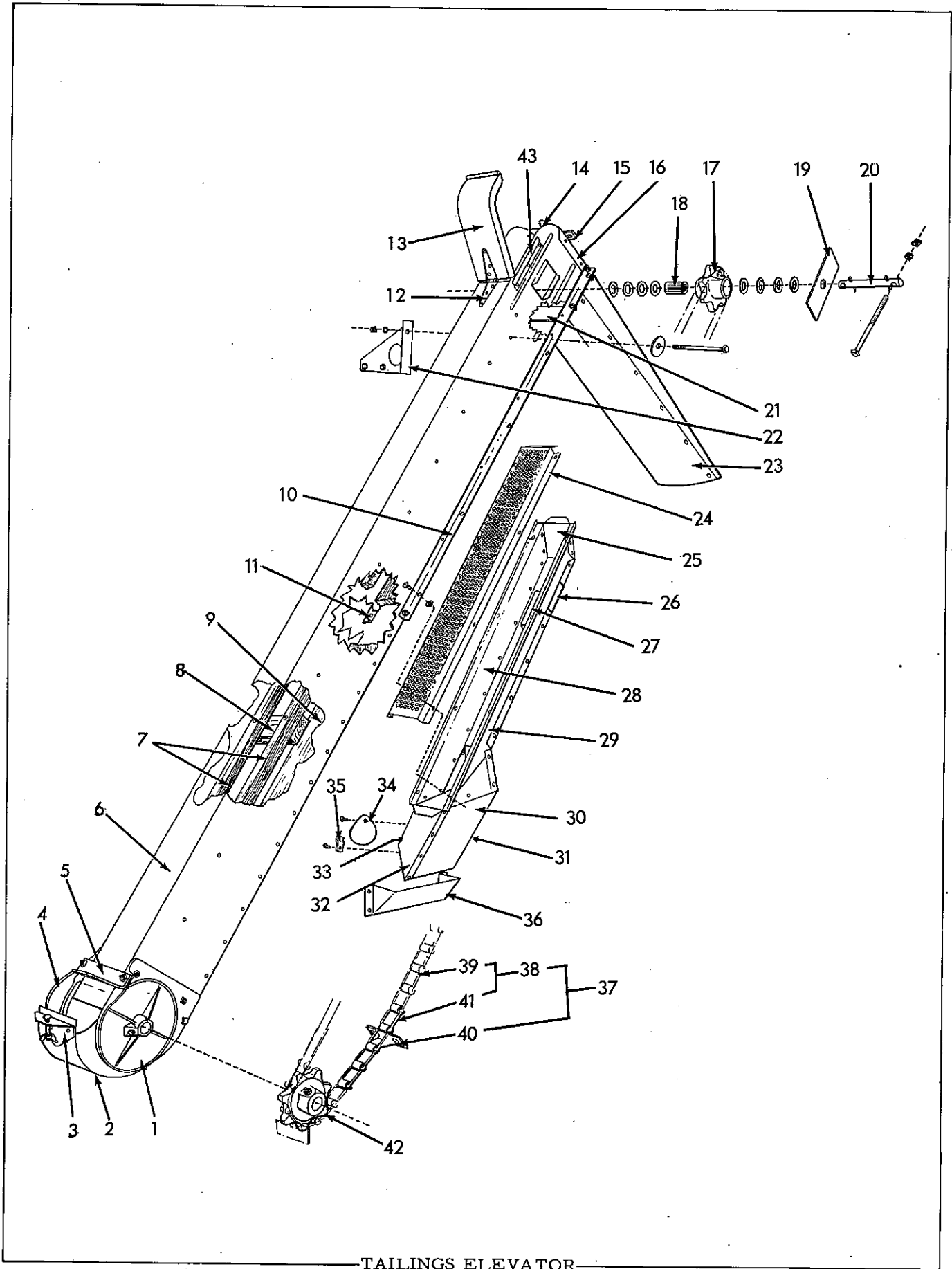
TAILINGS ELEVATOR
