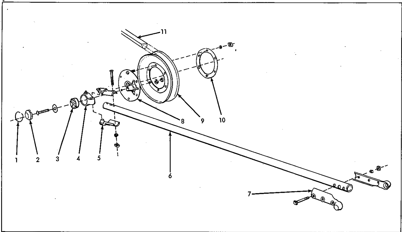
SICKLE DRIVE
