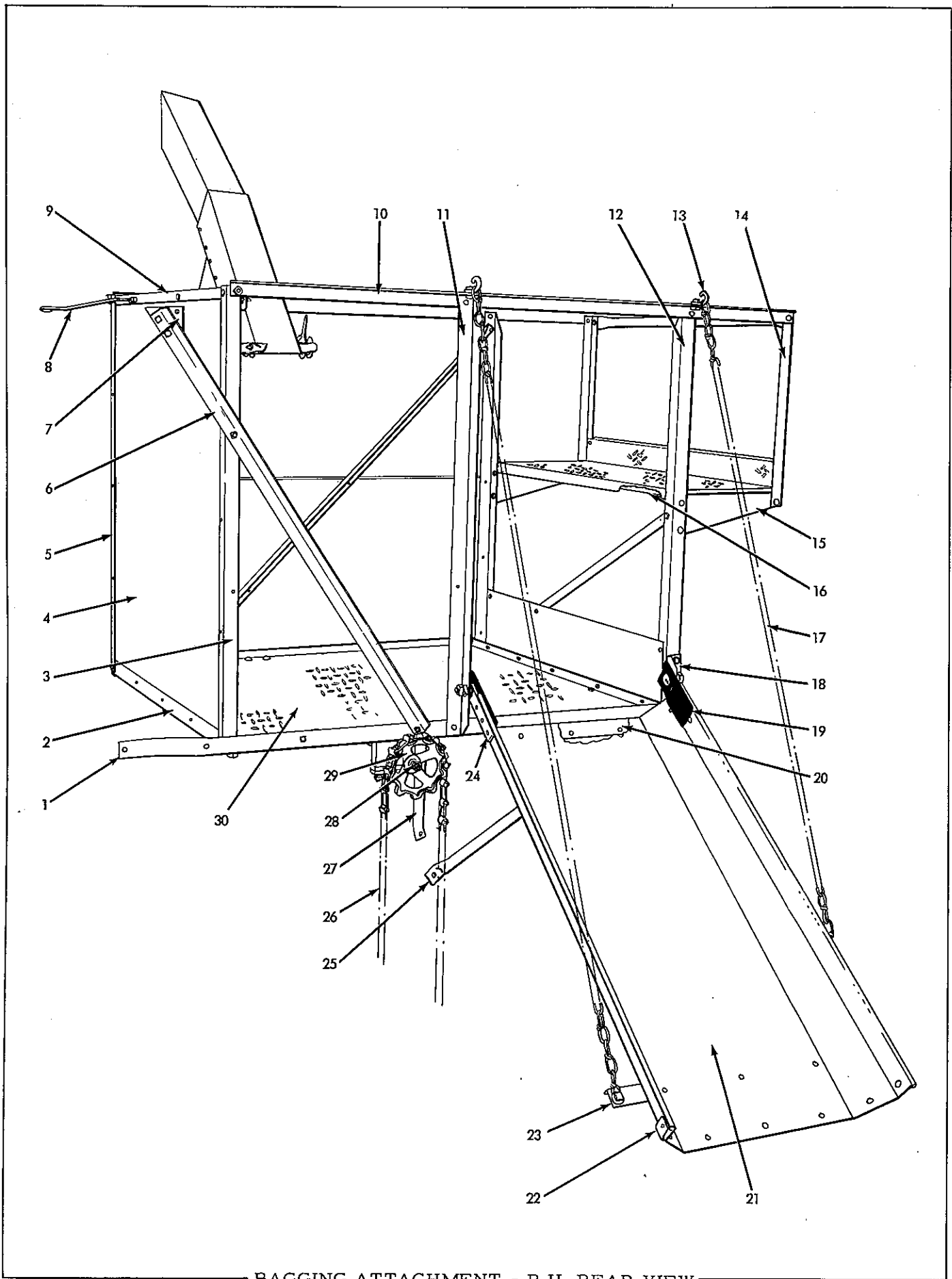
BAGGING ATTACHMENT - R.H. REAR VIEW
