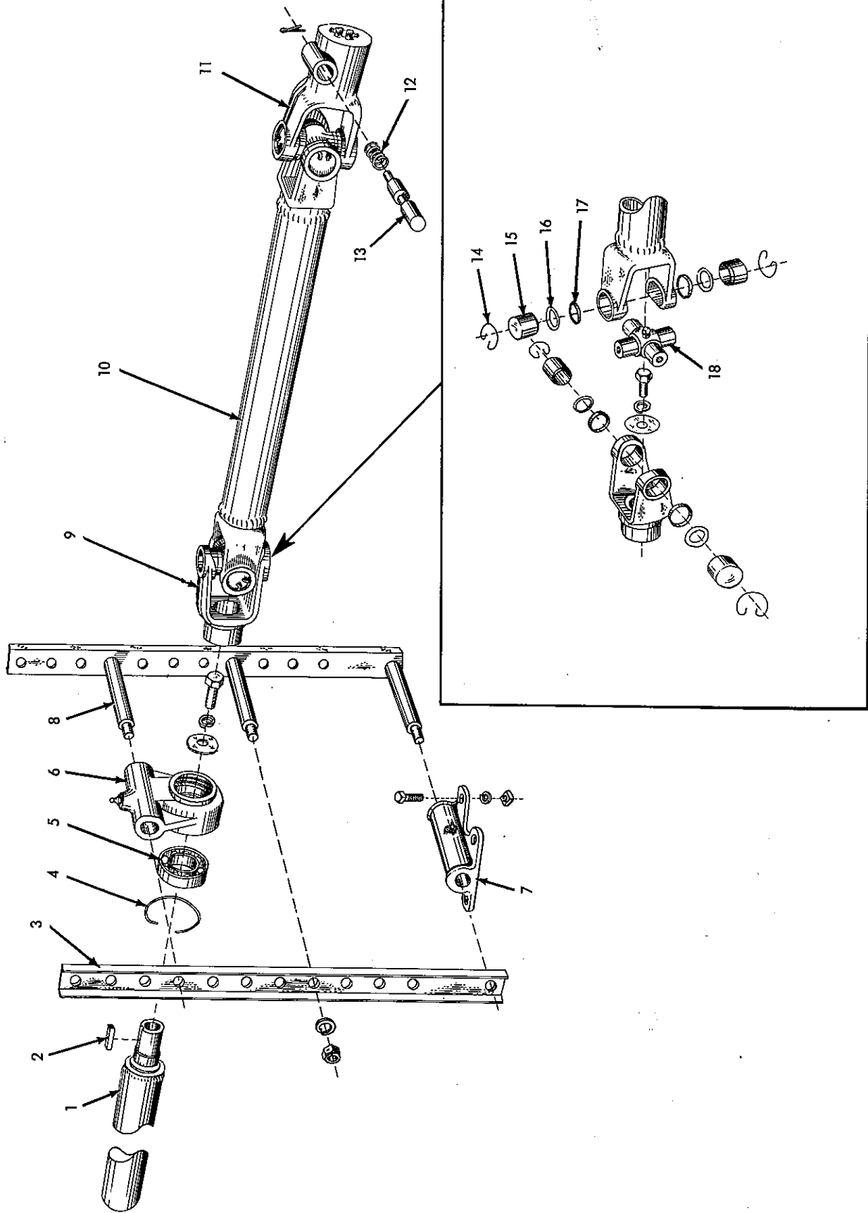
POWER TAKE-OFF SHAFT
