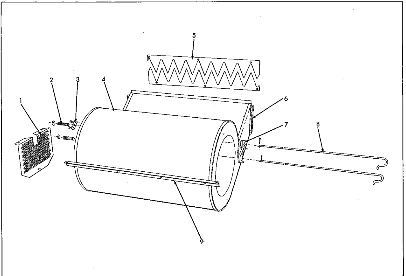
FAN HOUSING
