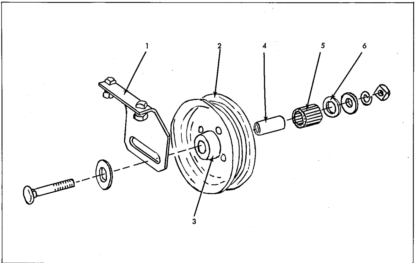
BIN CONVEYOR IDLER
