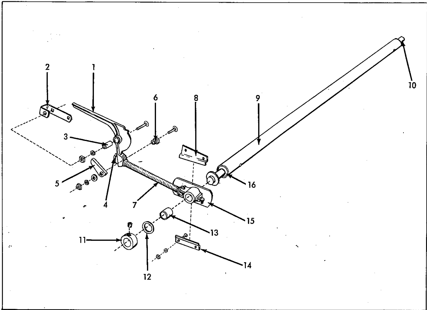
LOWER DRAPER IDLER ROLLER
