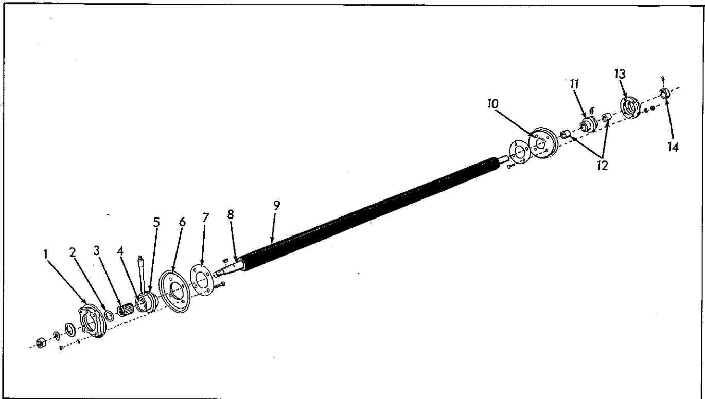
LOWER DRAPER DRIVE ROLLER
