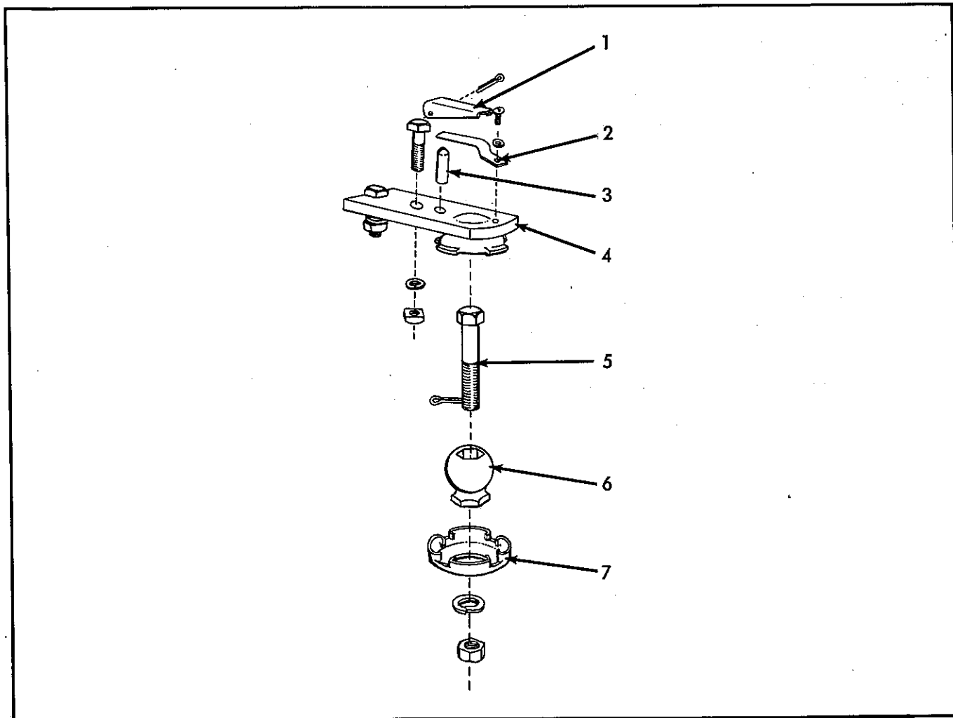
HITCH BALL & SOCKET
