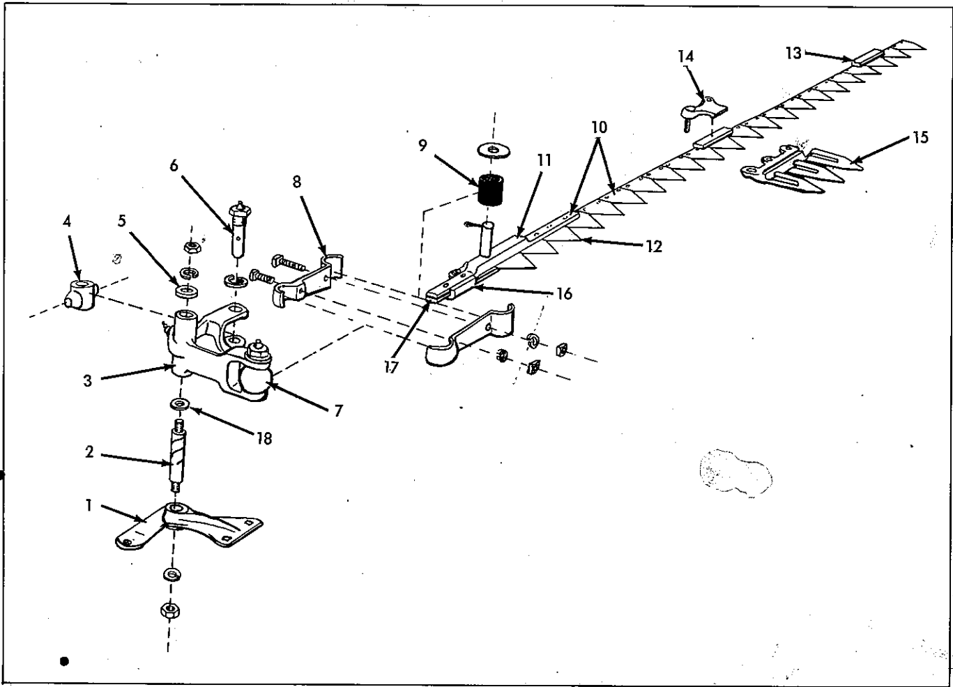
SICKIE & BELL CRANK
